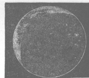
Fig 159. The Crescent.
