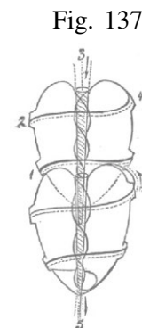
Fig. 137. Polarized Atoms.
