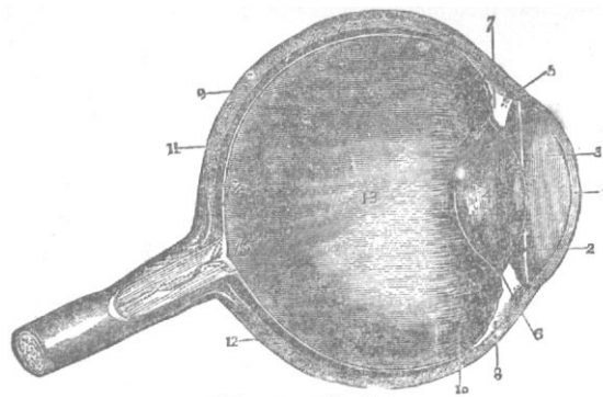
Fig. 197. The Eye.
