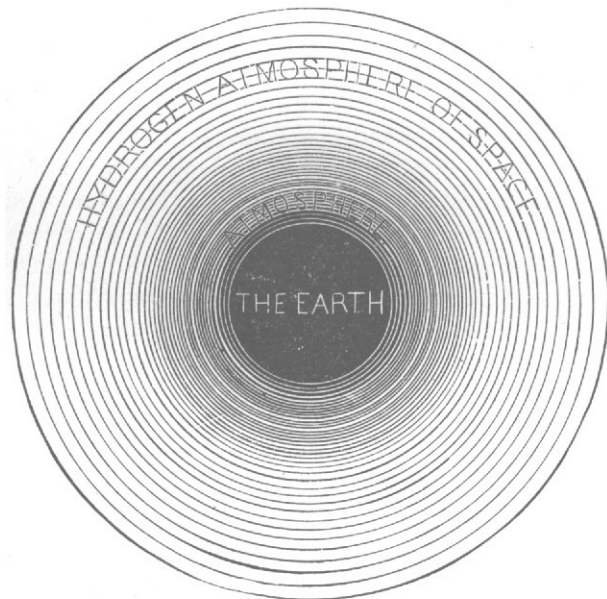
Fig. 152. The Ethereal Atmosphere of Space.
