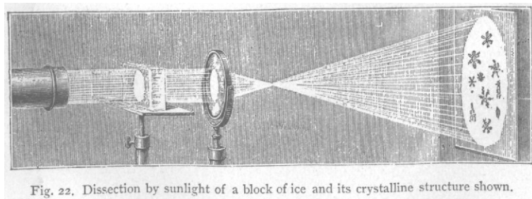
Fig. 22. Dissection by sunlight of a block of ice and its crystalline structure shown.
